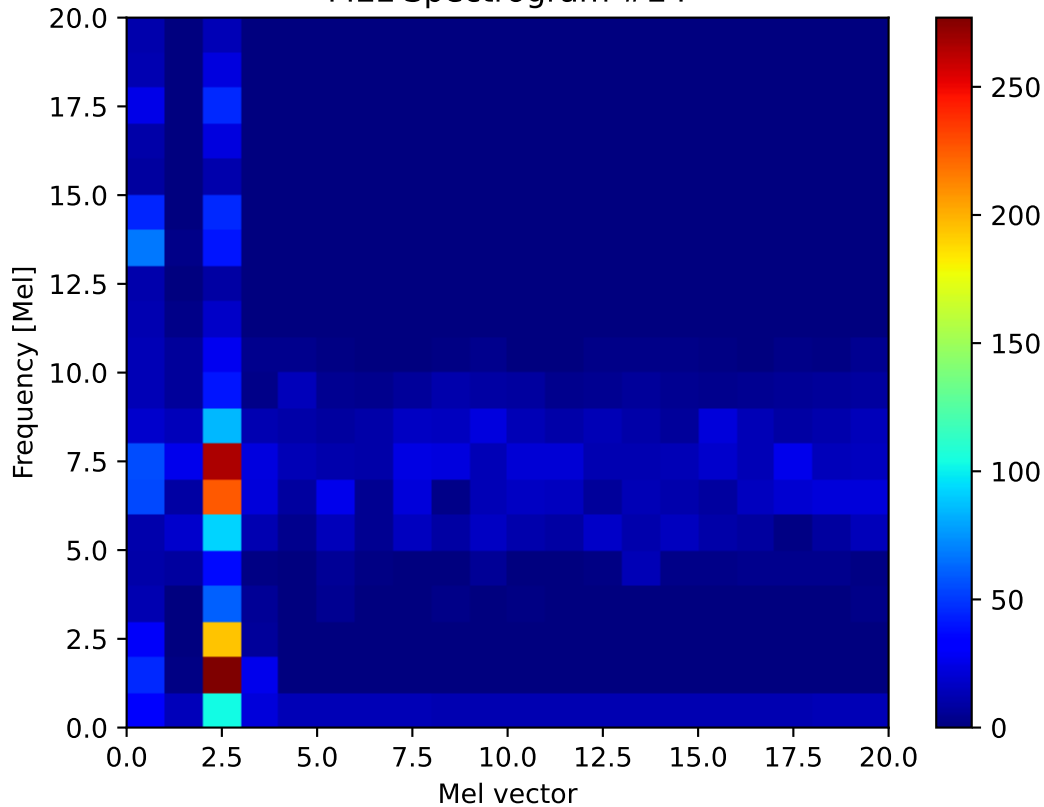
MEL Spectrogram #24
